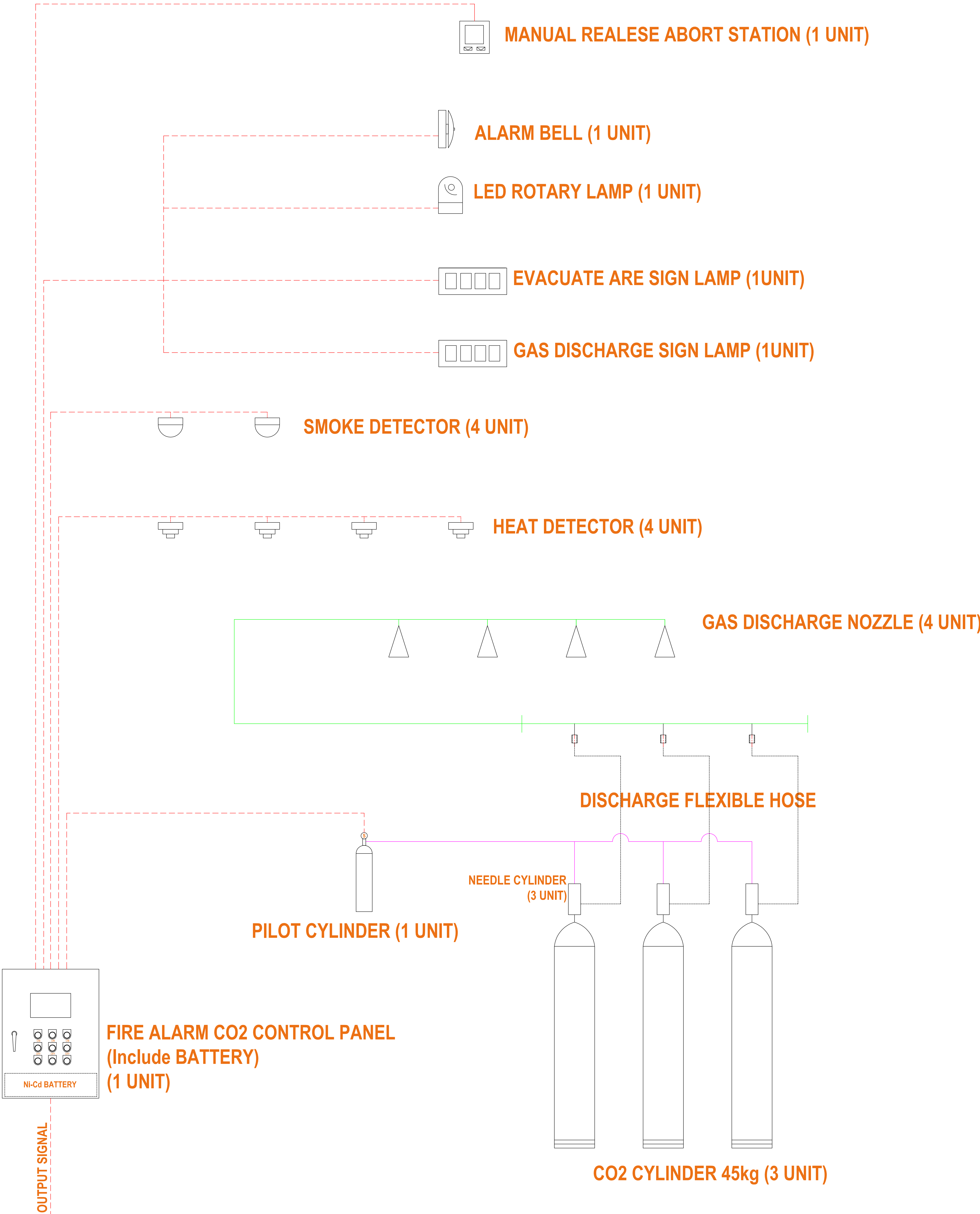
FLOW DIGRAM CO2 - FIRE FIGHTING SYSTEM
